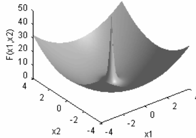
Figure 10. Misleading problem for evolutionary algorithms
