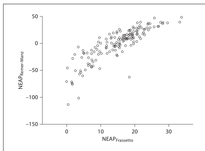
Fig. 1. Comparison of the two estimates of acid-base balance in vegan diets (SV and MV combined; r=0.873 , p < 0.001 ).
