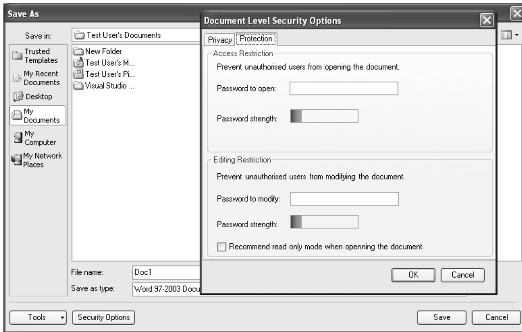
Figure 1: The Save As dialog in (a) original form with General Options dialog from the Tools button and (b) modified form with Document Level Security Options dialog from a new Security Options button
