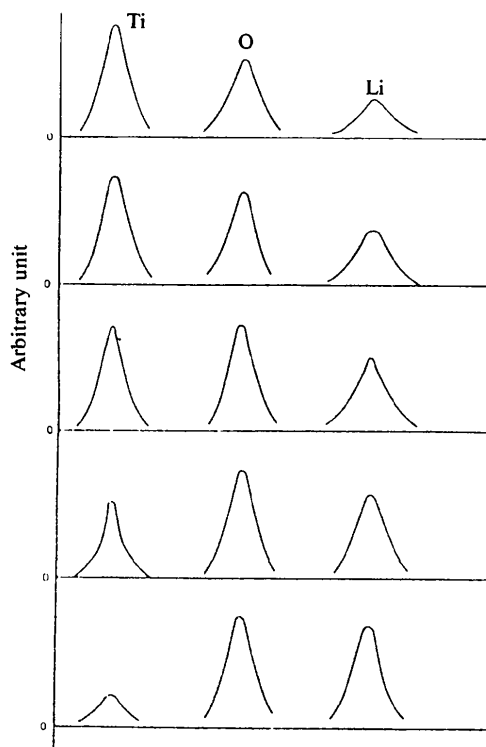
Fig. 2. Schematic diagram showing the relative variation of the image contrast for atoms of Ti, O and Li with crystal thickness. The increase of crystal thickness, successively from top to bottom in the diagram, leads to an enhancement of the image contrast of the light atom Li.
