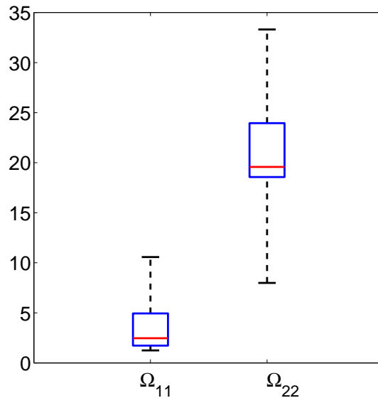
Figure 2 Inefficiency factors in the estimation of the TVP-VAR model of the US economy (see online version for colours)
