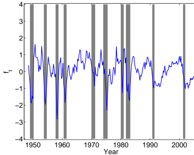
Figure 3 Estimated factor in the dynamic factor VAR model of the US economy together with the timing of officially announced US recessions (shaded regions) (see online version for colours)
