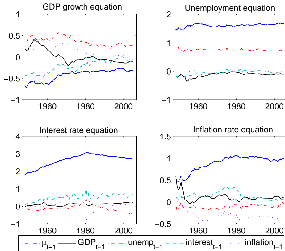
Figure 1 Evolution of the parameters \beta_t in the TVP-VAR model (see online version for colours)
