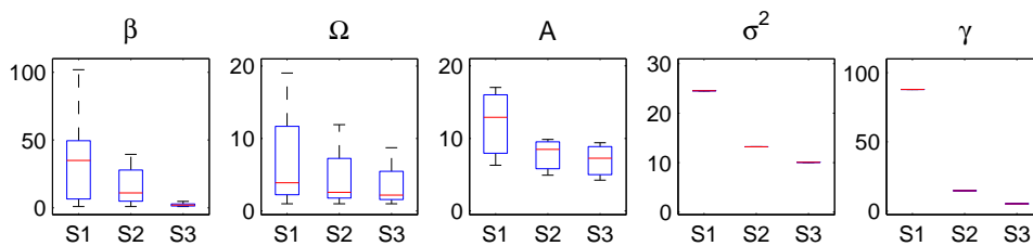
Figure 4 Inefficiency factors for the three sampling schemes (S1, S2, S3) in the DF-VAR model (see online version for colours)
