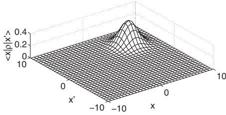
FIG. 6. Plot of \langle x|\rho|x' \rangle for a coherent state |\alpha\rangle , where \alpha=2.5 .
