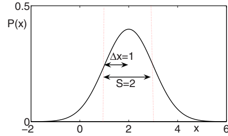
FIG. 4. (Color online) P(x) for a coherent state |\alpha\rangle : \Delta x = \Delta p = 1 .
