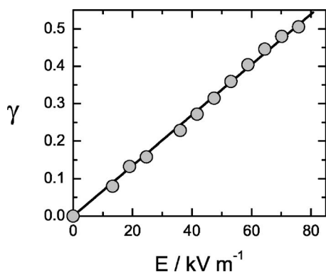
FIG. 8. The field dependence of the force ratio \gamma . \gamma was obtained by fitting the autocorrelations displayed in Fig. 7 to Eq. (19). The linear variation of \gamma with the field E confirms that the charge on the particle is independent of the strength of the applied field. The solid line yields an effective charge of |Z_{\text{eff}}| = 14.5 \pm 0.2 .
