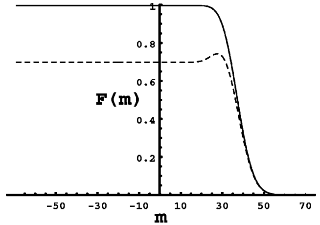
FIG. 2. The fidelity versus the result m for the number difference operator N_T - N_A for a coherent state in the target with \alpha = 6, \lambda = 0.9 (dashed) and \alpha = 6.0, \lambda = 0.99 (solid).
