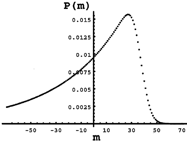
FIG. 1. The probability distribution for obtaining a result m for the number difference operator N_T - N_A for a coherent state in the target with \alpha = 6.0, \lambda = 0.99 .
