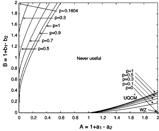
FIG. 7. Quantum copier properties which allow improvements in information transfer when using detectors of very low efficiency \eta having no dark counts ( \xi=0 ). A and B are parameters of the copiers, and the lines show boundaries of the regions in (A, B) space within which copiers give improvements. Various lines correspond to various a priori input photon probabilities p indicated on the plot. Improvements occur in the regions away from the diagonal A=B relative to the boundary lines for a given p . For higher efficiencies \eta , smaller regions of A-B parameter space are useful. The UQCM is indicated by the cross at (A, B)=(5/3, 1/3) , and the Wootters-Zurek copier by the circle at (2, 0) .
