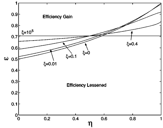
FIG. 4. Regions of efficiency gain for the single-copier ( N=1 ) detection scheme, as a function of \varepsilon , the copier, and \eta , the detector efficiencies, for varying frequency of dark counts parametrized by \xi . In all cases, the copier produces vacuum when it fails ( \mu=-1 ) and the input is equiprobable to be a photon or vacuum ( p=1/2 ).
