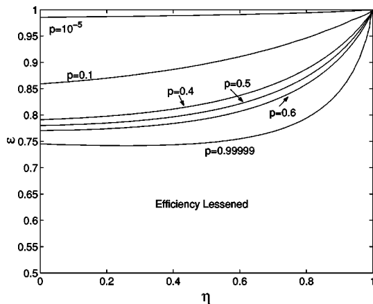
FIG. 6. Regions of efficiency gain for the single-copier ( N = 1 ) detection scheme, as a function of \varepsilon , the copier, and \eta , the detector efficiencies, for varying a priori photon input probabilities p . In all cases, the probability of dark counts in the detectors is taken to be zero ( \xi = 0 ), and the default output upon copy failure is a totally random state ( \mu = 0 ). Note that the scale in \varepsilon differs from that in Figs. 2, 4, and 5.
