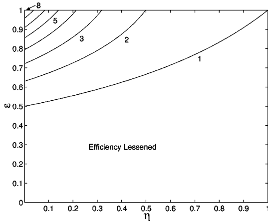
FIG. 2. Relative efficiency gain \eta^e / \eta contours for the three-level ( N=3 ) copier detection scheme over the basic detector ( N=0 ), as a function of detector efficiency \eta and copier efficiency \varepsilon , where both detectors and copiers are noiseless ( \xi=0, \mu=-1 ). Valid for any photon input probabilities p .
