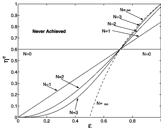
FIG. 3. Equivalent efficiency \eta^e , as a function of copier efficiency \varepsilon and number of levels of copiers N , when detector efficiency is \eta=0.6 , and both detectors and copiers are noiseless ( \xi=0, \mu=-1 ). Results for N=0-3 are shown as solid lines, and the limit of what can be achieved is shown as a dashed line. Regions beyond the N=0 and N \rightarrow \infty cases are not achievable with noiseless copiers. Valid for all photon input probabilities p .
