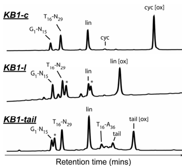
Figure S1. Incubation of cyclotide substrates with JB VPE. The KB1-c, KB1-l and KB1-tail peptides were incubated with JB VPE \pm 10 mM DTT at 30°C. RP-HPLC traces of the reaction mixtures after 16 hours are shown with the identity of the digestion products determined by mass labelled. All species are in the reduced form unless otherwise stated. Asterisks indicate proteins that could not be identified.
