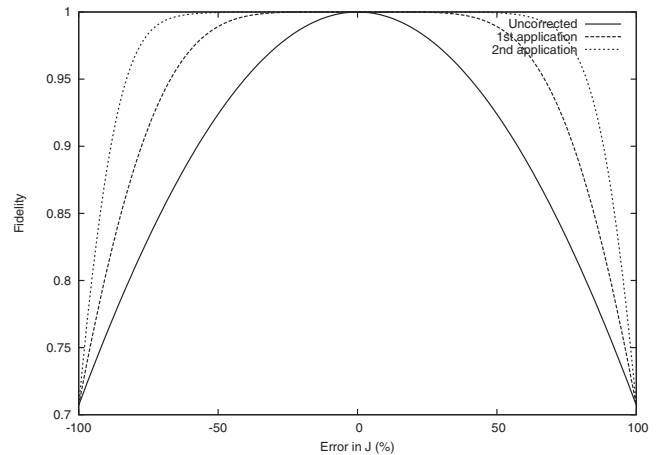
FIG. 1. This plot shows the fidelity of several methods of creating a CNOT gate, with a systematic error in the strength of the coupling.
