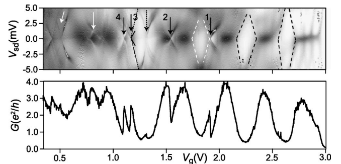
FIG. 4. (a) Differential conductance ( dI/dV_{sd} ) versus bias voltage ( V_{sd} ) and gate voltage ( V_g ). Dark correspond to high (maximum= 4e^2/h ) and white to low conductance. Fano resonances are indicated with the arrows. (b) Corresponding linear response conductance G .
