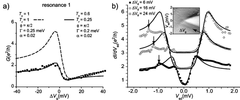
FIG. 6. Comparison between the measured differential conductance of the Fano resonance 1 [see Fig. 4(a)] and fits to Eq. (3). In (a) the solid curve represents the best fit taking into account only the linear response conductance, whereas the dashed curve is calculated from average parameters deduced by fitting the nonlinear differential conductance dI/dV_{sd} vs V_{sd} for a set of (only) positive gate voltages, shown in (b). The curves are vertically offset by e^2/h for clarity. For (a) the whole set of parameters are given in the figure, whereas the parameters for the three fits in (b) are \blacksquare : T_n=0.85 , T_r=0.9 , \Gamma=0.25 meV, \phi=\pi/2 , and \alpha=0.027 ; \square : T_n=1 , T_r=1.2 , \Gamma=0.25 meV, \phi=\pi/2 , and \alpha=0.02 ; \circ : T_n=1.1 , T_r=1.4 , \Gamma=0.25 meV, \phi=\pi/2 , and \alpha=0.017 . The observed asymmetry in bias voltage originates from different coupling of the resonant states to the leads. The inset in (b) shows the measured differential conductance. An excited state is visible for V_{sd} < 0 , both in the grayscale plot and the dI/dV_{sd}(V_{sd}) (arrows).
