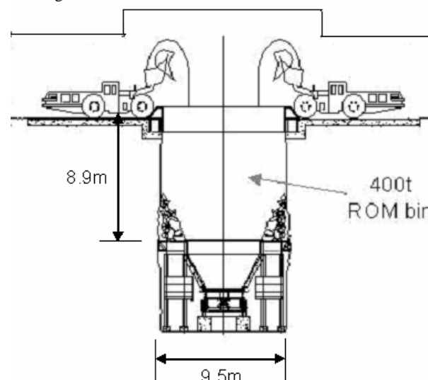
Fig.1 Typical LHD trucks tipping into a ROM bin
