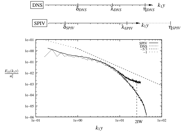
Figure 7: Longitudinal spectra of v at y^+ = 100 , with an inner scaling
