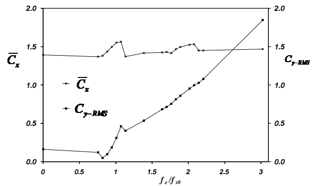
Figure 13 – Mean and fluctuating force coefficients for 60° forced oscillations, Re=80, A/D=0.14 .
