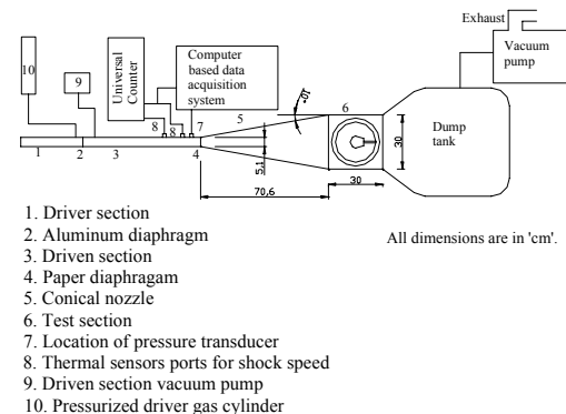
Figure 1: Layout of IISc hypersonic shock tunnel, HST2.
