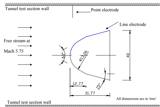
Figure 7: Schematic diagram of blunt cone model with electrode arrangement for flow visualization experiment.
