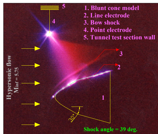
Figure 8: Shock structure around the blunt cone model.
