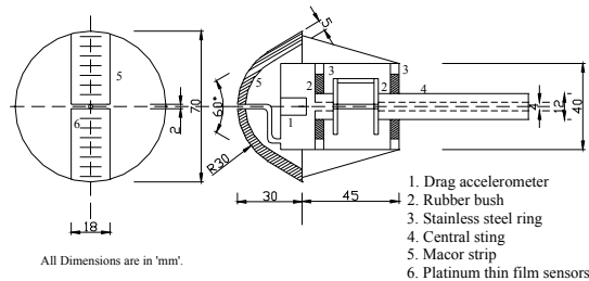
Figure 2: A 60^\circ apex-angle blunt cone model fitted with an accelerometer balance system and platinum thin film gauges for simultaneous drag and heat transfer measurements.
