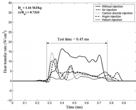
Figure 5: Numerically integrated heat transfer signal for platinum thin film sensors 'with and without' gas injection.
