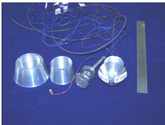
Figure 3: Photograph of the 60^\circ apex-angle blunt cone model along with an accelerometer balance system and platinum thin film gauges for simultaneous drag and heat transfer measurements.
