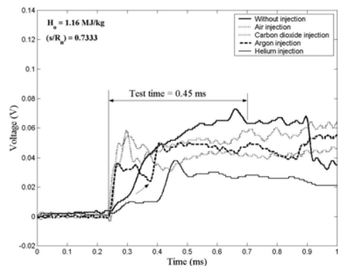
Figure 4: Typical temperature-time history from platinum thin film sensors 'with and without' gas injection.
