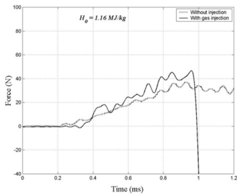
Figure 6: Typical force-time history inferred from drag accelerometer at 0° angle of attack.
