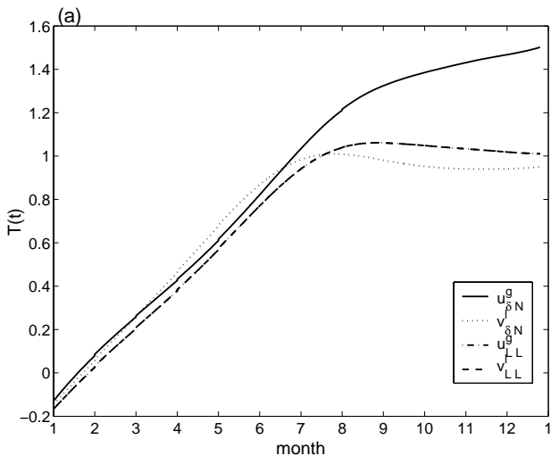
Figure 7. Comparisons between El Niño and La Niña events. u_{\delta N}^g(u_{LN}^g) : the SSTA nonlinear (linear) evolution of the CNOP (the corresponding LSV), and v_{\delta N}^g(v_{LN}^g) : the SSTA nonlinear (linear) evolution of -T (negative anomaly of SST) of the local CNOP (the corresponding LSV). This figure is from [6].
