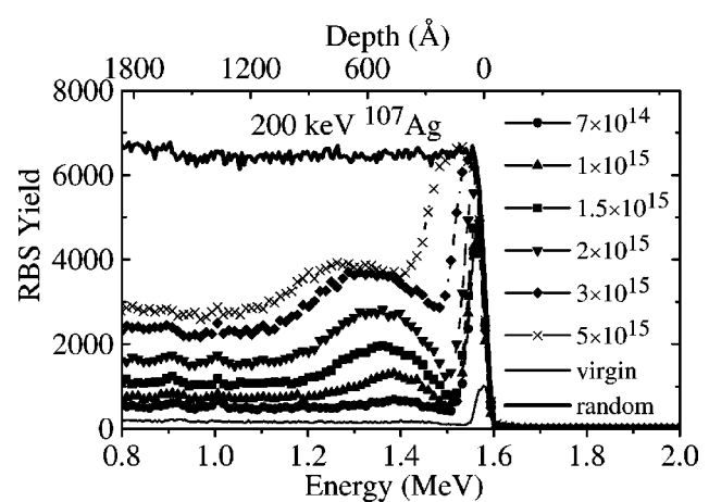
FIG. 5. RBS/C spectra showing the damage buildup for 200 keV Ag ion bombardment of GaN at 20^\circ\text{C} with a beam flux of 6.0 \times 10^{11} \text{ cm}^{-2} \text{ s}^{-1} . Implantation doses (in \text{cm}^{-2} ) are indicated in the figure.
