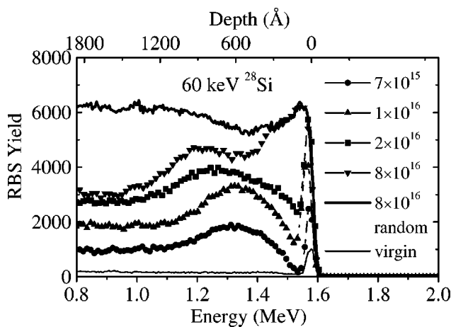
FIG. 3. RBS/C spectra showing the damage buildup for 60 keV Si ion bombardment of GaN at 20^\circ\text{C} with a beam flux of 1.6 \times 10^{13} \text{ cm}^{-2} \text{ s}^{-1} . Implantation doses (in \text{cm}^{-2} ) are indicated in the figure.
