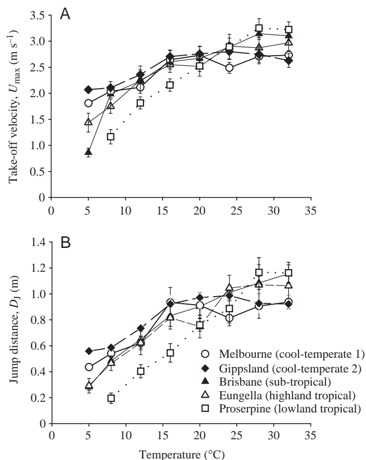
Fig. 2. Thermal sensitivity of (A) maximum take-off velocity ( U_{\max} ) and (B) maximum jump distance ( D_J ), for adult striped marsh frogs ( Limnodynastes peronii ) from five populations across a wide geographic range. The relationship between temperature and each parameter of jumping performance was significantly different amongst the populations (two-way repeated-measures ANOVA) ( P < 0.05 ). Values are means ± S.E.M. (Melbourne, N=12 ; Gippsland, N=24 ; Brisbane, N=22 ; Eungella, N=13 ; Proserpine, N=14 ).
