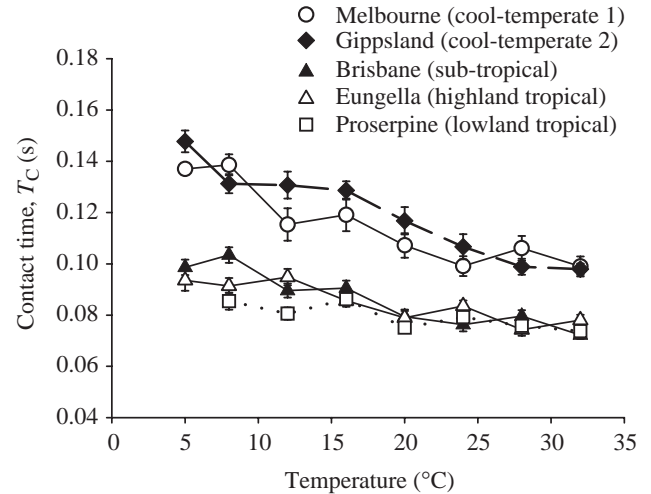
Fig. 4. Thermal sensitivity of contact time on the platform during a jump ( T_C ) for adult striped marsh frogs ( Limnodynastes peronii ) from five populations across a wide geographic range. The relationship between temperature and T_C was significantly different amongst the populations (two-way repeated-measures ANOVA) ( P < 0.05 ). Values are means \pm S.E.M. (See Fig. 2 for N values.)
