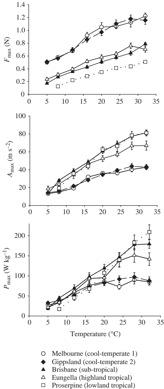
Fig. 3. Thermal sensitivity of (A) maximum jumping force ( F_{\max} ), (B) maximum jumping acceleration ( A_{\max} ) and (C) maximum instantaneous jumping power ( P_{\max} ) for adult striped marsh frogs ( Limnodynastes peronii ) from five populations across a wide geographic range. The relationship between temperature and both parameters of jumping performance was significantly different amongst the populations (two-way repeated-measures ANOVA) ( P < 0.05 ). Values are means \pm S.E.M. (See Fig. 2 for N values.)
