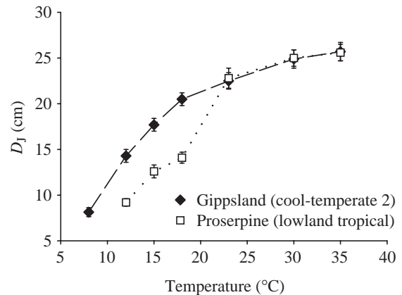
Fig. 5. Thermal sensitivity of maximum jump distance ( D_J ) for metamorph striped marsh frogs ( Limnodynastes peronii ) raised under identical conditions in the laboratory from the cool-temperate Gippsland and lowland tropical Proserpine population. Thermal sensitivity of D_J differed significantly between the two populations (two-way repeated-measures ANOVA) ( P < 0.05 ). Values are means \pm S.E.M. (Gippsland, N=19 ; Proserpine, N=13 ).
