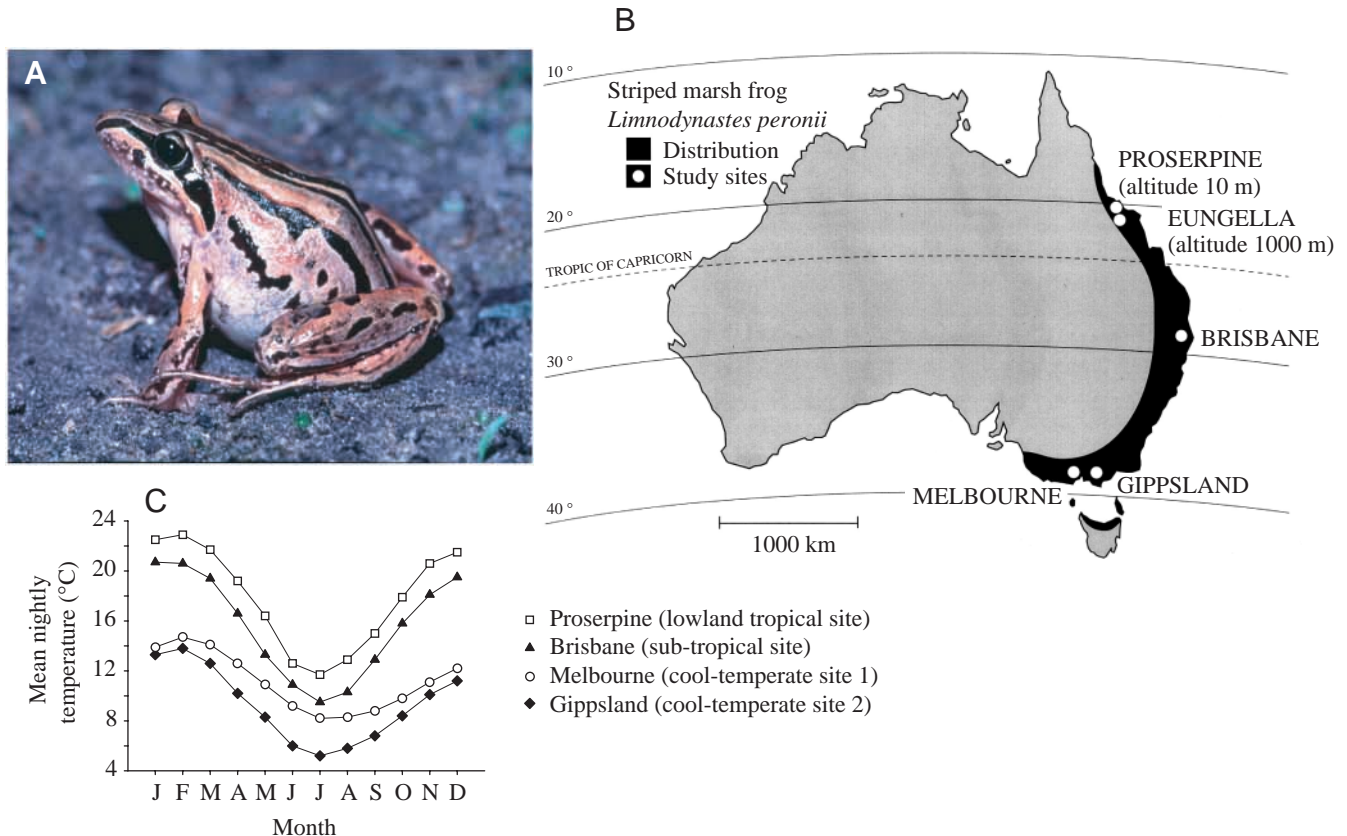
Fig. 1. (A) A striped marsh frog ( Limnodynastes peronii ) (photograph courtesy of E. Meyer). (B) Distribution of striped marsh frogs along the eastern regions of Australia. Symbols indicate sites where adult animals were collected. (C) Seasonal changes in average nightly temperature at four of the study sites (Australian Bureau of Meteorology).
