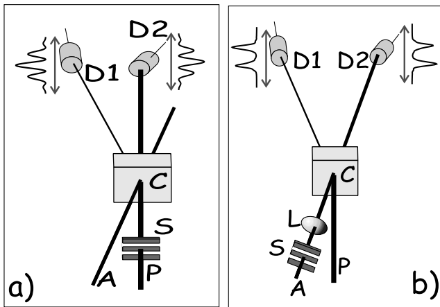
FIG. 1. Sketch of the experiment. P is the pump beam, A is the auxiliary beam, S is the double slit, L is the lens, C is the nonlinear crystal, and D1 and D2 are detectors. (a) Slits inserted in the pump beam. (b) Slits and lens inserted in the auxiliary beam.
