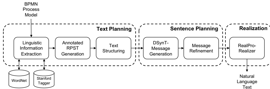
Abb. 1: Architecture of our Natural Language Generation System
