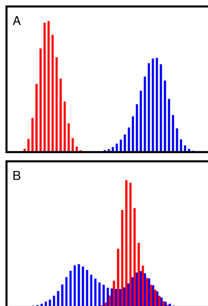
Figure 2.8: Histogram comparisons.
