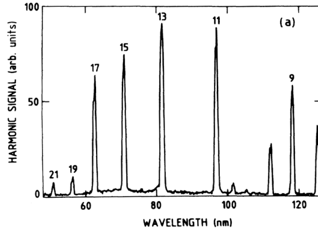
Figure 1.7: High-order harmonic spectrum. One of the first demonstrations of HHG in a xenon gas jet by using 1064 nm, picosecond laser pulses. Graph is taken from Ref. [19]. ©1989 APS.
