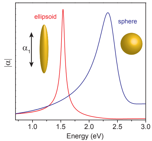
Figure 1.10: Absolute value of the polarizability |\alpha| for a small gold sphere and a gold ellipsoid with high aspect ratio. Shown are the calculated polarizabilities for a sphere and an antenna-like ellipsoid with respect to the excitation frequency of the driving light wave (expressed in eV). The dielectric function \epsilon_{Au}(\omega) was fitted with an analytic model for the optical properties of gold [44].
