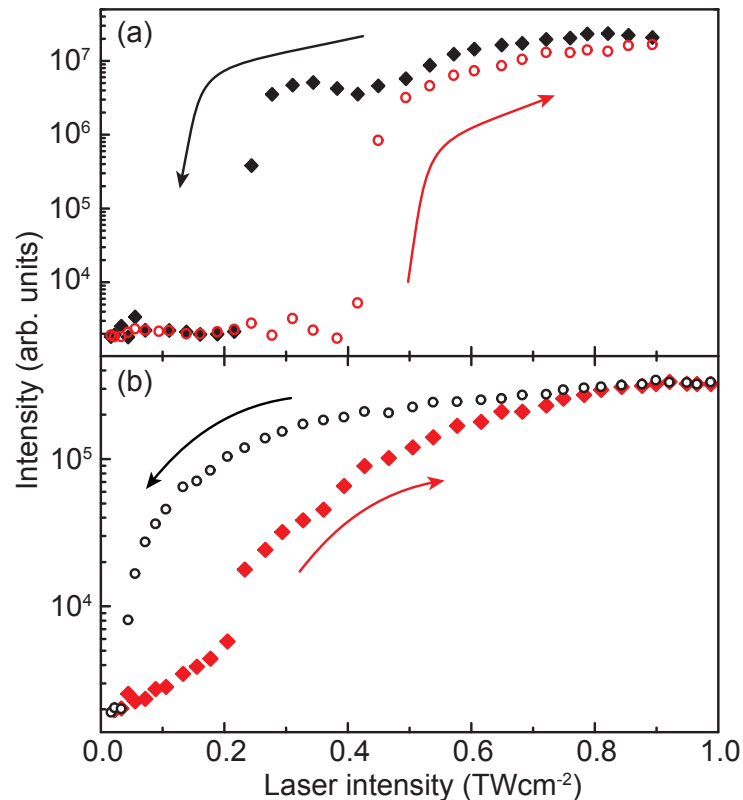
Figure 5.7: Intensity hysteresis from a fresh and moderately modified waveguide. a) Hysteresis measurement using a fresh waveguide with smooth inner surface right after the fabrication process. Same data as shown in Fig. 4.4(a). (b) Hysteresis measurement for the same waveguide as in (a), but with moderately modified surface roughness caused by illumination with laser intensities in the excess of 1 TW/cm 2 .
