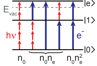
Figure 5.5: Ionization paths.
