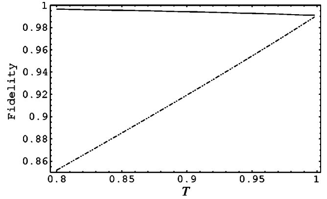
FIG. 1. The fidelity between the photon-subtracted state and the ideal coherent-state superposition with an ideal single-photon detector (solid line) and a threshold detector (dotted line). The initial squeezing parameter is \exp(2s) = 2.36 and the x axis is the transmittivity of the beam splitter T = t^2 . The amplitude \alpha of the ideal coherent-state superposition is optimized for the maximum fidelity. The optimized amplitude \alpha ranges between 1.02 (when T = 0.8 ) and 1.16 (when T \rightarrow 1 ).
