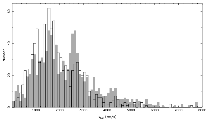
FIG. 25.—Histogram of the H I systemic velocities, v_{\text{sys}} , of the HIPASS BGC galaxies ( white ). For comparison we overlaid ( in gray ) the optical velocity histogram of the 1000 optically brightest galaxies obtained from LEDA (see § 5).
