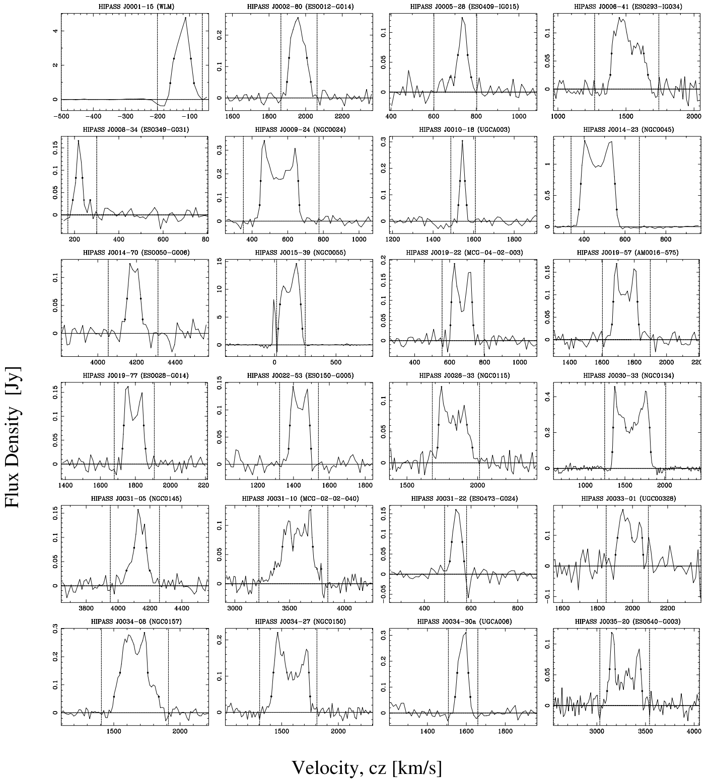
FIG. 1.—H I spectra of all 1000 members of the HIPASS Bright Galaxy Catalog (BGC). The HIPASS name together with the most likely optical identification (in brackets) is given at the top of each spectrum. The measured H I peak flux density as well as the 50% and 20% velocity widths are also marked. The vertical lines indicate the velocity range used for the first-order baseline fit ( outside ) and the H I line emission analysis ( inside ). [See the electronic edition of the Journal for 40 additional panels.]
