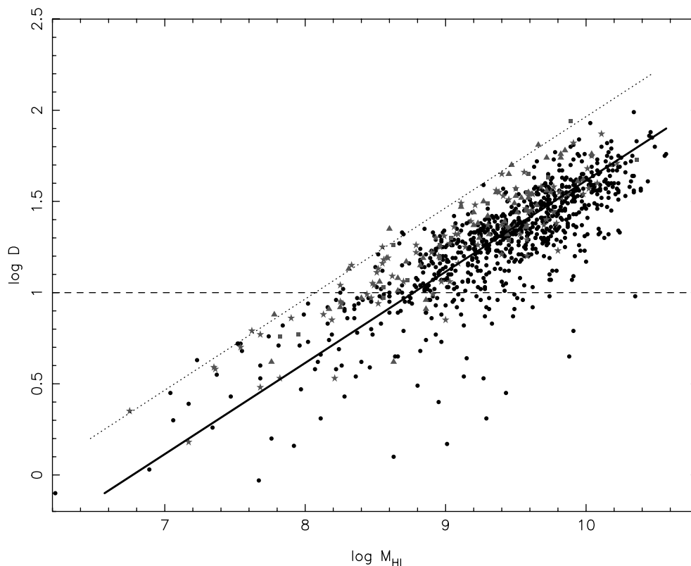
FIG. 16.—Derived distances D , of all HIPASS BGC sources vs. derived H I mass M_{\text{HI}} . The solid black line marks the F_{\text{HI}} -completeness limit ( F_{\text{HI}} = 25 \text{ Jy km s}^{-1} ), while the dotted line denotes the approximate detection limit, F_{\text{HI}} = 5 \text{ Jy km s}^{-1} , of the BGC. The horizontal dashed line indicates a distance of D = 10 \text{ Mpc} . Newly cataloged galaxies as well as H I clouds are marked with stars, galaxies with previously unknown velocities with triangles, and galaxies with previously incorrect velocities with squares. In total there are 157 (248) galaxies with v_{\text{LG}} < 750 ( 1000 \text{ km s}^{-1} ) of which 20 (27) are newly cataloged. For comparison, see Fisher & Tully (1981a) and Briggs (1997).
