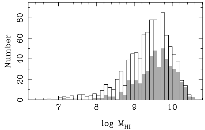
FIG. 15.—Histogram of the H I mass, M_{\text{HI}} , distribution in the HIPASS BGC. We show the full sample of 1000 sources ( white ) and the complete F_{\text{HI}} -limited subsample ( gray ) with F_{\text{HI}} > 25 \text{ Jy km s}^{-1} (see § 3.7).
