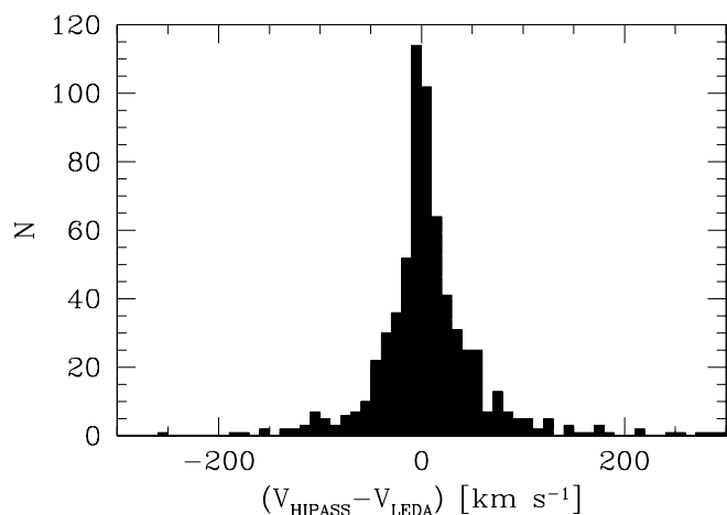
FIG. 6.—Histogram of the difference between the H I and optical systematic velocities for 672 HIPASS BGC objects. For 95% of these galaxies, the optical velocities are within 170 \text{ km s}^{-1} of the HIPASS velocities. There are 20 galaxies with differences larger than 300 \text{ km s}^{-1} ; these lie outside the velocity range displayed here.
