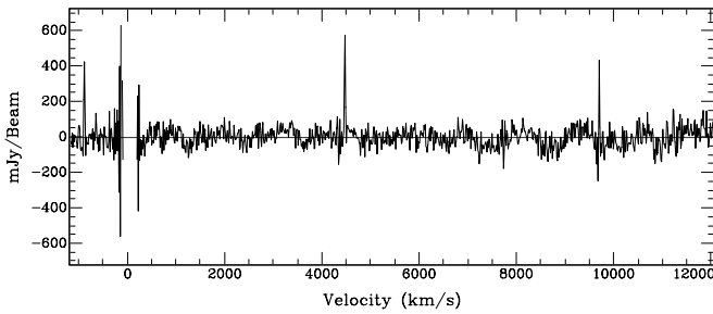
FIG. 11.—Example of strong Galactic recombination lines in HIPASS, here shown at the position of the H II region complex IC 4701. In this case three narrow lines are visible at velocities of -890 , 4465 , and 9690 \text{km s}^{-1} . The Galactic emission around 0 \text{km s}^{-1} has mostly been blanked out.
