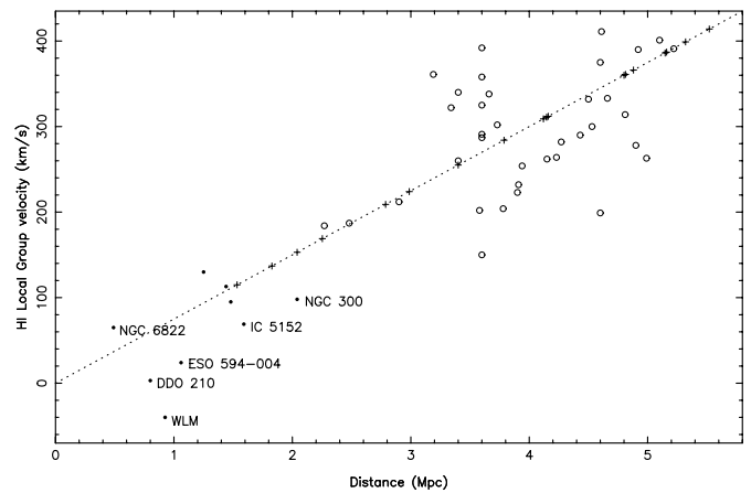
FIG. 3.—Distances vs. H I Local Group velocities for the closest galaxies in the BGC. Open and filled circles indicate galaxies for which independent distances are available in the literature (see § 3.4.2), while crosses denote the Hubble distance ( D = v_{LG}/H_0 ) for those galaxies for which no independent distances are currently available. The filled circles show those nine galaxies for which the independent distances were adopted in the BGC. The largest deviations occur when one distance is given for members of a galaxy group (e.g., part of the Cen A group at 3.6 Mpc, see Karachentsev et al. 2003).
