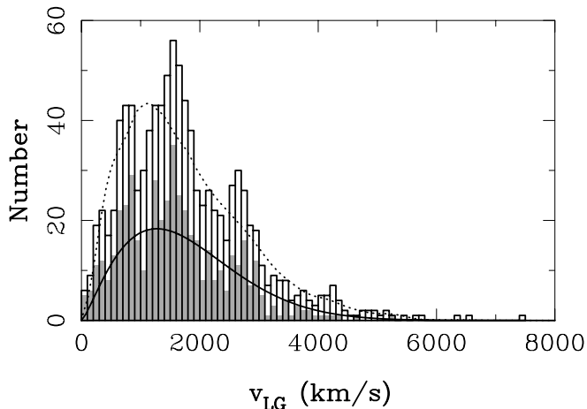
FIG. 13.—Histogram of the H I Local Group velocities, v_{\text{LG}} , in the HIPASS BGC. We show the full sample of 1000 sources (white) and the complete F_{\text{HI}} -limited subsample (gray) with F_{\text{HI}} > 25 Jy km s -1 (see § 3.7). Overlaid are the selection functions for both samples as derived by Zwaan et al. (2003).
