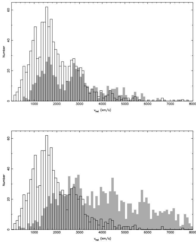
FIG. 14.—Histogram of the H I systemic velocities, v_{\text{sys}} , of the HIPASS BGC galaxies ( white ). For comparison we overlaid ( in gray ) the H I velocity histograms from the targeted samples of Mathewson et al. (1992) ( top ) and Theureau et al. (1998) ( bottom ) selecting only southern galaxies with H I velocities less than 8000 \text{ km s}^{-1} . The samples contain 569 and 1188 galaxies, respectively.
