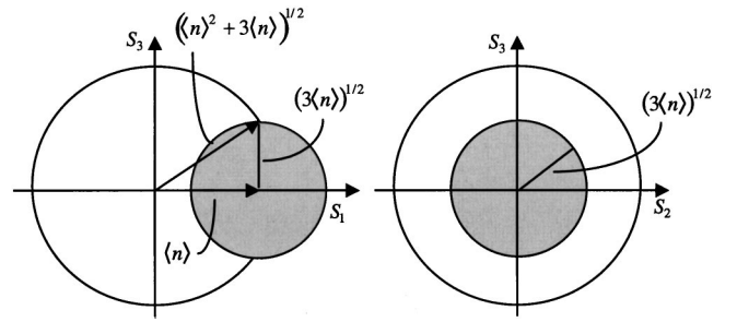
FIG. 2. Sections of the Poincaré sphere in the 3,1 and 2,3 planes for the x -polarized coherent state. The shaded disks show the projections of the uncertainty sphere of the Stokes vector in these planes.
