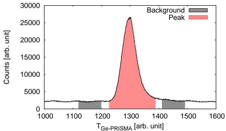
Figure 3.18: Ge-PRISMA coincidence time spectrum for \theta_{PRISMA} = 54^\circ .
