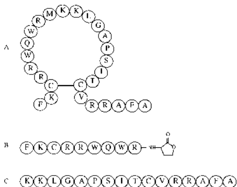
FIG. 5. The primary sequence of lactoferricin and CNBr-derived subfragments. The peptides were identified by N-terminal sequencing and MS. (A) Lactoferricin, differing from lactoferricin B (7) by the presence of a C-terminal alanine residue. (B) Subfragment 1, including the C-terminal homoserine lactone. (C) Subfragment 2.
