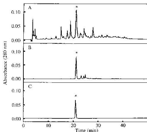
FIG. 4. Analytical RP-HPLC of ion-exchange and preparative HPLC fractions of pepsin-hydrolyzed Lf that contain lactoferricin. Samples were brought to 0.1% TFA and 10 \mu l was injected onto a Vydac C 18 column (25 by 0.46 cm [i.d.]; solvent A, 0.1% TFA; solvent B, 90% acetonitrile in 0.09% TFA; equilibration was in 20% solvent B for 5 min; gradient, 20% solvent B to 50% solvent B over 40 min; flow rate, 1 ml/min). (A) Pepsin-hydrolyzed Lf. (B) Ion-exchange fraction containing lactoferricin. (C) RP-HPLC-purified lactoferricin. The elution position of lactoferricin is indicated with asterisks.
