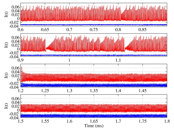
FIG. 12. Control to period 1 using nonsubtractive feedback of the FIR laser with A \approx 0.05 . The average pulsation period before and during control is 1.179\mu\text{s} and 0.9747\mu\text{s} , respectively. The intensity is in arbitrary units.
