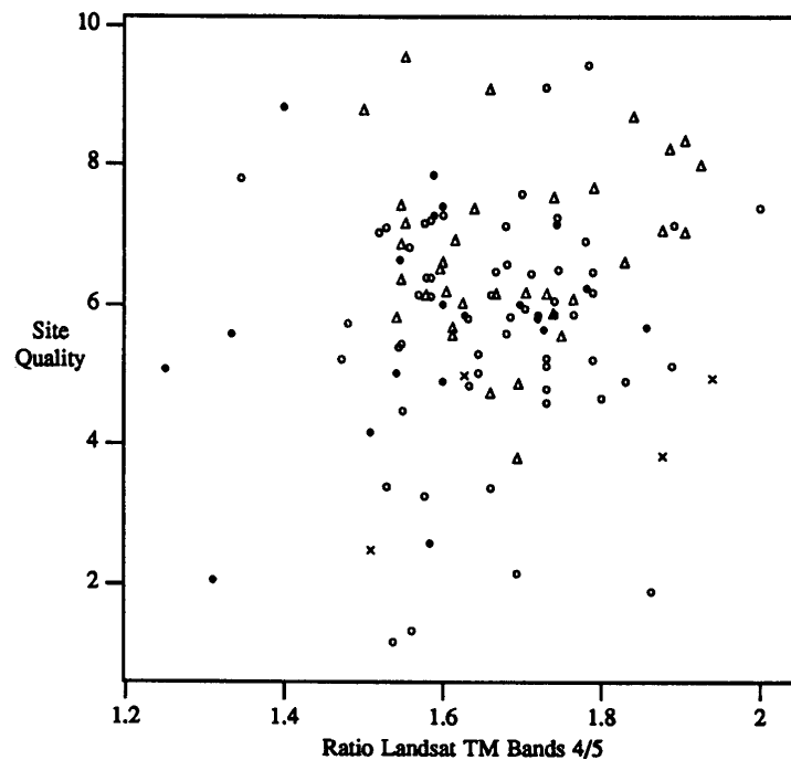
FIG. 2. Scatterplot of site quality and ratio of bands 4/5 (October 1987). (× acid volcanic, ○ basic volcanic, Δ coarse granite, ● sedimentary metamorphic)
