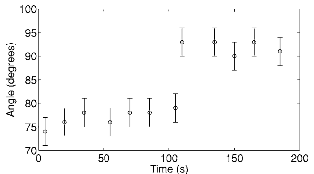
FIG. 3. Change in orientation of a growing lysozyme crystal. The angle between the optic axis of the crystal and the beam axis is shown.
