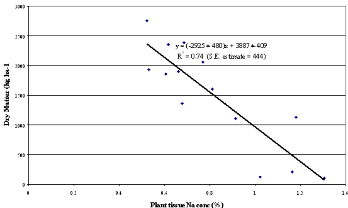
Figure 2 The relationship between dry matter (kg ha -1 ) and Na tissue concentration (%) of the lucerne whole tops.
