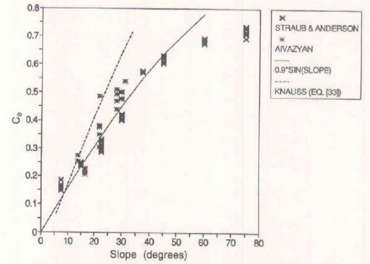
Fig. 8 - Uniform equilibrium air concentration C_e as a function of the spillway slope
