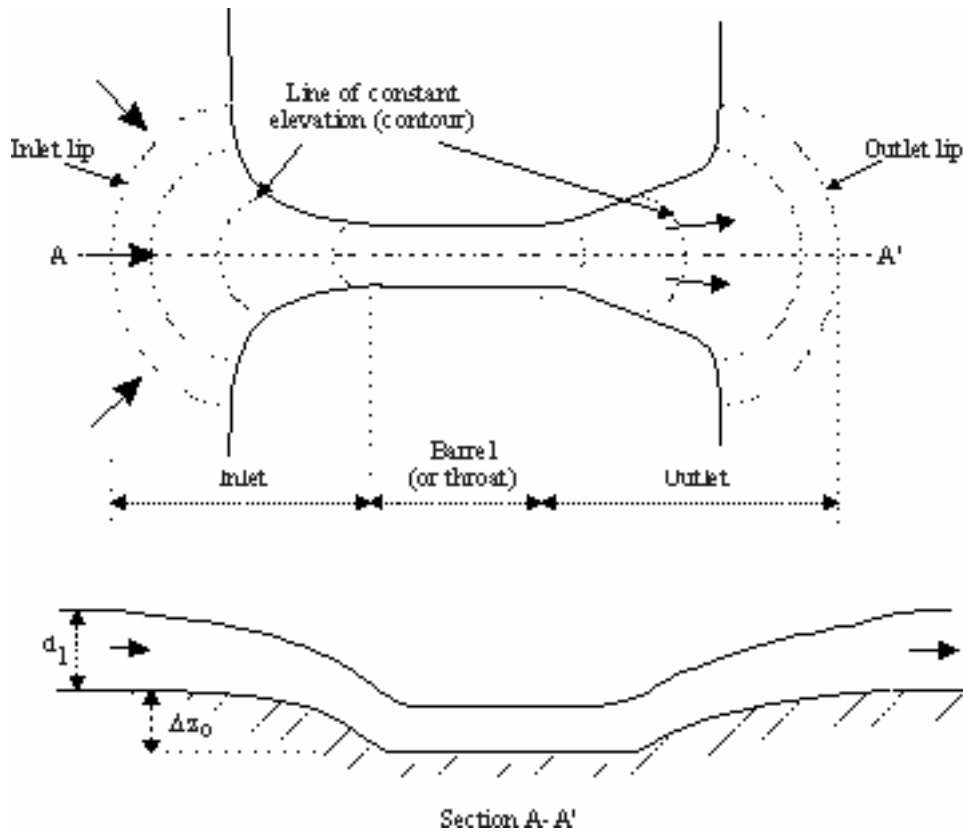
Fig. 2 -- Sketch of a Minimum Energy Loss culvert
