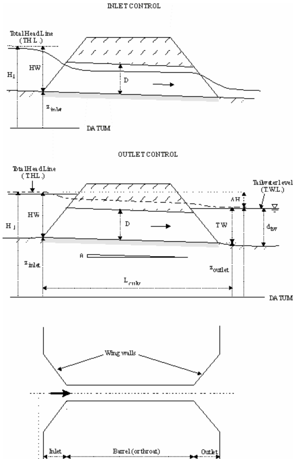
Fig. 1 - Sketch of a standard culvert operation : inlet control and outlet control
