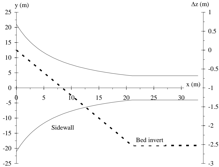
Figure 7 - MEL culvert design - Design parameters : Design flow rate = 100 \text{ m}^3/\text{s} - Barrel width : 8 m - Zero afflux - Normal depth in the flood plain (in absence of culvert) : d_0 = 1.2 \text{ m}
