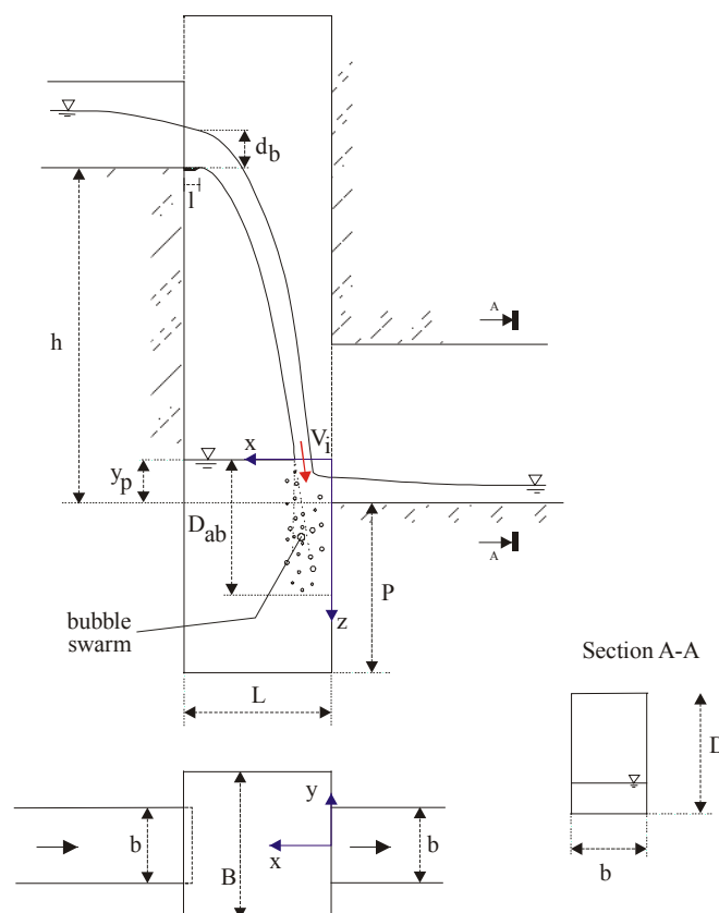
Fig.1 - Definition sketch of rectangular dropshafts
