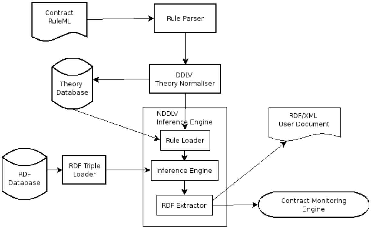
Figure 3. DR-CONTRACT System Architecture
