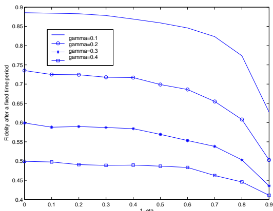
FIG. 3: Average fidelity after a fixed amount of time as a function of 1-efficiency for several error rates (parameters used: dt = 10^{-4} , \kappa = 50 , \lambda = 50 , r = 10 , T = 1500 \times dt ).
