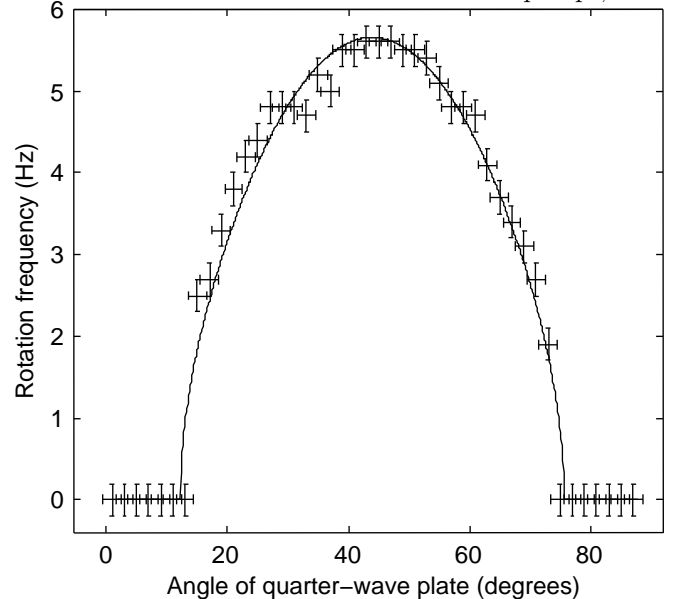
FIG. 4: The variation of rotation frequency with the polarization of the trapping beam. The sudden onset of rotation when the minimum angle is reached can be clearly seen. The theoretical response of the particle allows a particle of unknown size to be measured, or can be used to determine the viscosity of a fluid. In this case, the trapping beam has a power of 50 mW, and the particle is 6.15 \mu\text{m} in radius and 2.3 \mu\text{m} thick. The frequency of rotation for a trapping beam of power P and optical frequency \omega is f = [\text{Re}(P\{[1 - \cos kd(n_o - n_e)]^2 \sin^2 2\phi - \sin^2 kd(n_o - n_e) \cos^2 2\phi\}^{1/2})]/(2\pi\omega D) . The drag torque coefficient D can be estimated by representing the particle as an ellipsoid [6]. The drag will lie between that of a sphere of radius a in a medium of viscosity \mu ( D = 8\pi\mu a^3 ) and a disk of the same radius ( D = (32/3)\mu a^3 ). Under the very low Reynolds number flow conditions encountered here, the surface texture and fine structure of the particle are unimportant. The maximum rotation speed, f = P/\pi\omega D , will result when the incident light is circularly polarized and the particle is a half-wave plate. Small particles will generally rotate faster due to less drag, but as particles become too small, their thickness becomes much less than the ideal half-wave case, and they will not intercept all of the power available to spin larger particles.
