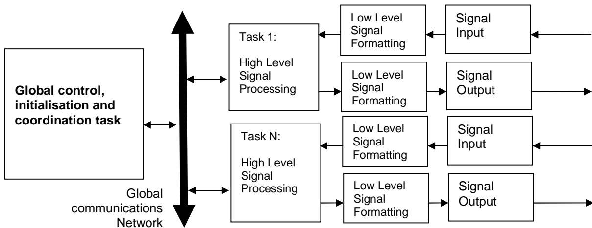
Figure 1: A Hierarchy of communicating real-time tasks
