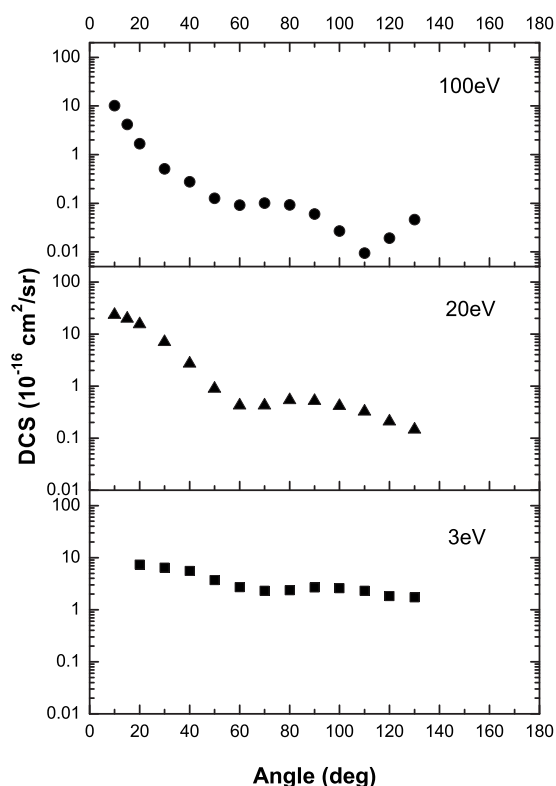
FIG. 27. Representative elastic differential cross sections for electron scattering from SiH 4 (in units of 10^{-16} cm 2 /sr).
