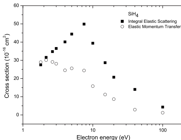
FIG. 28. Recommended integral elastic cross sections and momentum transfer cross sections for electron scattering from SiH 4 (in units of 10^{-16} cm 2 ).
