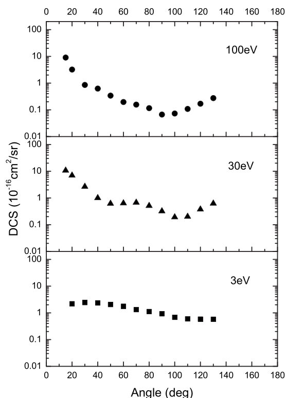
FIG. 23. Representative elastic differential cross sections for electron scattering from NF 3 (in units of 10^{-16} cm 2 /sr).
