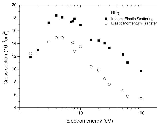
FIG. 24. Recommended integral elastic cross sections and momentum transfer cross sections for electron scattering from NF 3 (in units of 10^{-16} cm 2 ).
