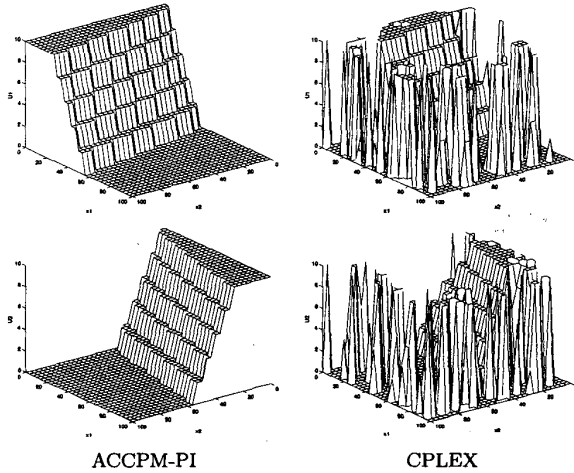
Figure 4: Optimal policy.
