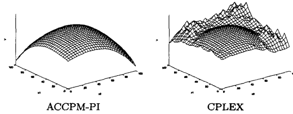
Figure 3: Value function.
