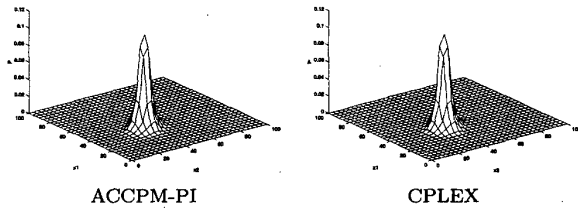
Figure 2: Steady state probability.
