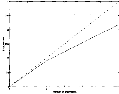
Figure 1: Speed-up as a function of the number of processors.
