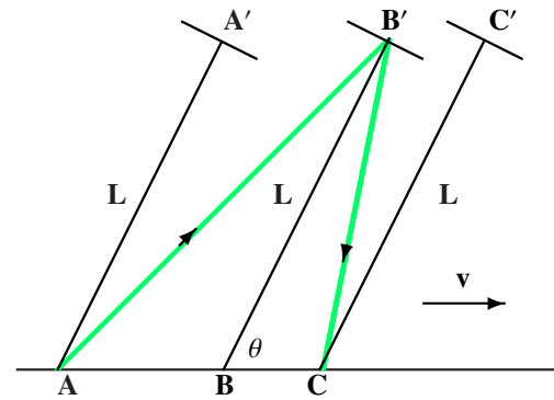
Fig. 4: Co-moving Earth-Moon-Earth photon bounce trajectories in reference frame of 3-space, so speed of light is c in this frame. Earth (APO) and Moon (retroreflector) here taken to have common velocity v wrt 3-space. When APO is at locations A,B,C, at times t_A, t_B, t_C, \dots the moon retroreflector is at corresponding locations A', B', C', \dots at same respective times t_A, t_B, t_C, \dots . Earth-Moon separation distance L , at same times, has angle \theta wrt velocity v , and shown at three successive times: (i) when photon pulse leaves APO at A (ii) when photon pulse is reflected at retroreflector at B' , and (iii) when photon pulse returns to APO at C.
