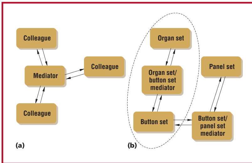
Figure 1. (a) The Mediator pattern; (b) a mediator and two colleagues (circled) in the Prism system.
