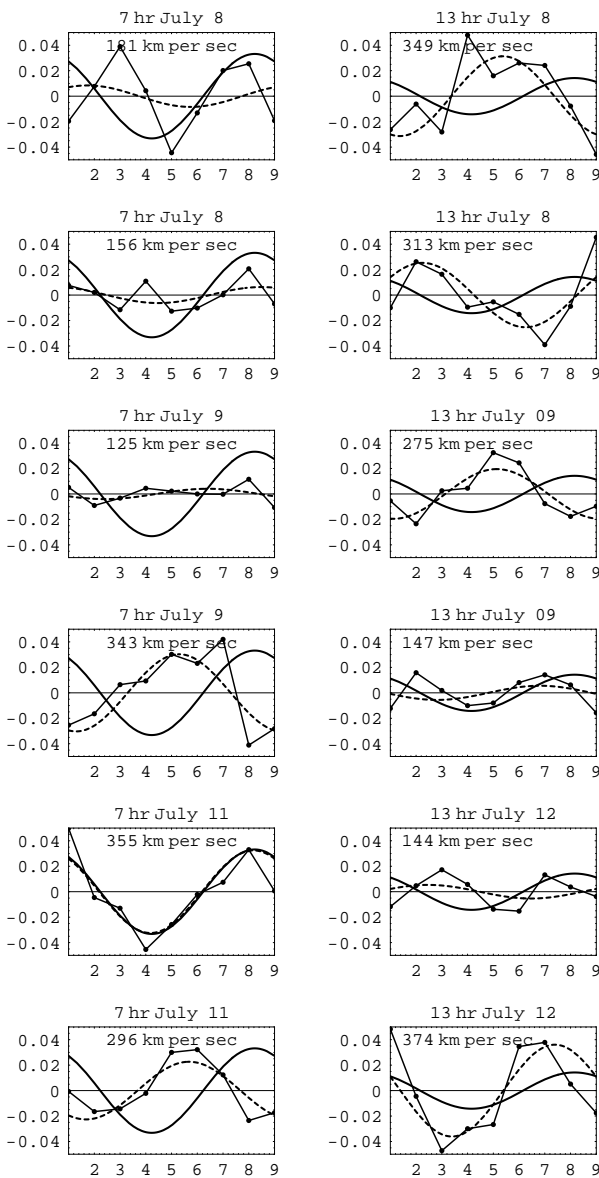
Fig. 2: Shows all the Michelson-Morley 1887 data after removal of the temperature induced linear fringe drifts. The data for each 360° full turn (the average of 6 individual turns) is divided into the 1st and 2nd 180° parts and plotted one above the other. The dotted curve shows a best fit to the data using (5), while the full curves show the expected forms using the Miller direction for \mathbf{v} and the location and times of the Michelson-Morley observations in Cleveland, Ohio in July, 1887. While the amplitudes are in agreement in general with the Miller based predictions, the phase varies somewhat. Miller also saw a similar effect. This may be related to the Hick's effect [4] when, necessarily, the mirrors are not orthogonal, or may correspond to a genuine fluctuation in the direction of \mathbf{v} associated with wave effects. We see that this data corresponds to a speed in excess of 300 km/s, and not the 8 km/s reported in [1], which was based on using Newtonian physics to calibrate the interferometer.
