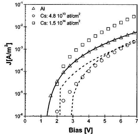
FIG. 5. Current density-voltage characteristics at various Cs deposition coverages: 4.8 \times 10^{13} (circle) and 1.5 \times 10^{14} (square) atoms/cm 2 and without Cs (triangle). For the latter structure the conductivity (solid line) is accurately described by the steady-state model. At a Cs coverage of 4.8 \times 10^{13} atoms/cm 2 we calculated the effect of a hole trapping level (upper dashed line) or an electron donor level (lower dashed line).
