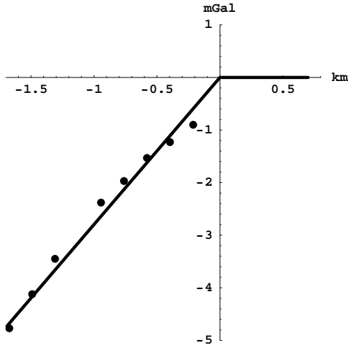
Figure 1: The data shows the gravity residuals for the Greenland Ice Cap [3] Airy measurements of the g(r) profile, defined as \Delta g(r) = g_{Newton} - g_{observed} , and measured in mGal ( 1\text{mGal} = 10^{-3} \text{ cm/s}^2 ), plotted against depth in km. Using (28) we obtain \alpha^{-1} = 139 \pm 5 from fitting the slope of the data, as shown.
