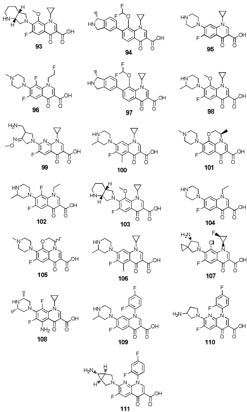
Figure 28. Chemical structures of the fluoroquinolone and quinolone classes of antibiotics with antichlamydial activity.
