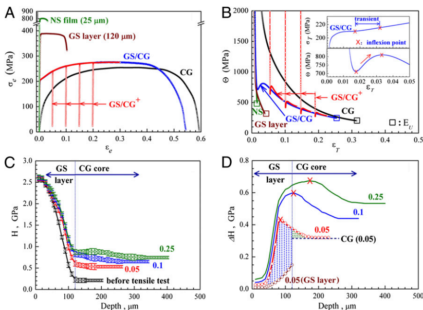
Fig. 2. Hardening rate up-turn and unique extra strain hardening. (A) Tensile engineering stress-strain ( \sigma_e - \varepsilon_e ) curves at a quasistatic strain rate of 5 \times 10^{-4} \text{ s}^{-1} . CG: standalone homogeneous CG sample; GS layer: grain-size GS layer of 120- \mu\text{m} thickness; GS-CG: sandwich sample of 1-mm thickness. NS: freestanding, quasihomogeneous nanostructured film of 20- \mu\text{m} thickness peeled from the top surface of GS; GS-CG + : the same sandwich sample subjected to unloading-reloading tensile testing at four separate strains of 0.05, 0.1, 0.15, and 0.2. All tensile samples were dog-bone-shaped, with a gauge dimension of 8 mm \times 2.5 mm. (B) Strain hardening rate ( \theta = d\sigma/d\varepsilon ) vs. true strain ( \varepsilon_T ) curves. (Inset) Transient response on the \sigma_T - \varepsilon_T curve of the GS-CG sample between two inflection points marked by "x," corresponding to the \theta -up-turn on its \theta - \varepsilon_T curve. GS-CG + (red curve) shows \theta -up-turn upon each reloading. (C) Vickers microhardness ( H_v ) vs. depth. The H_v values were measured on the cross-sectional GS-CG sample after tensile testing them to varying strains (labeled on the curves). The border between GS layer and CG core is located at 120- \mu\text{m} depth. (D) \Delta H ( H increment) vs. depth after varying tensile strains. The dotted area indicates the extra hardening in the GS-CG sample.
