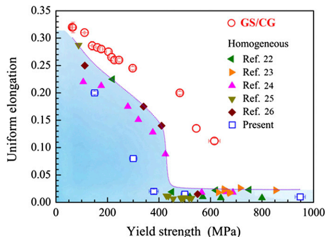
Fig. 5. Superior mechanical property. Strength and ductility in the GS-CG samples of IF-steel compared with their homogeneous counterparts.
