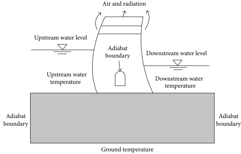
FIGURE 2: Boundary conditions of a dam.
