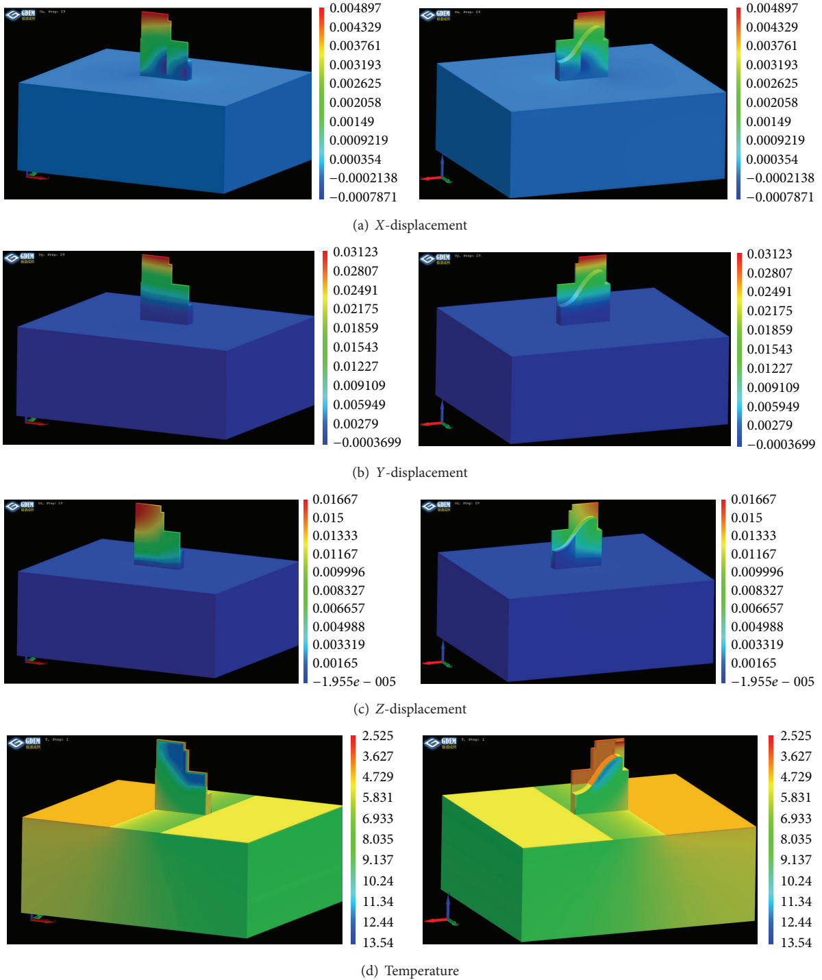
FIGURE 8: The simulation results using the GPU parallel solver.
