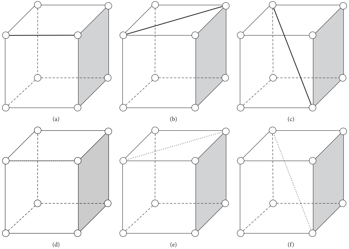
FIGURE 1: Definitions and connection types of 1d element.
