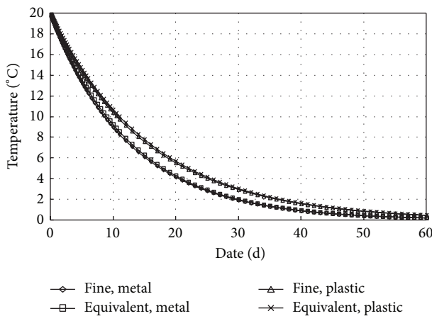
FIGURE 4: Comparison between the fine and equivalent models.
