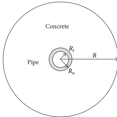
FIGURE 3: The model of a cylinder water cooling pipe.
