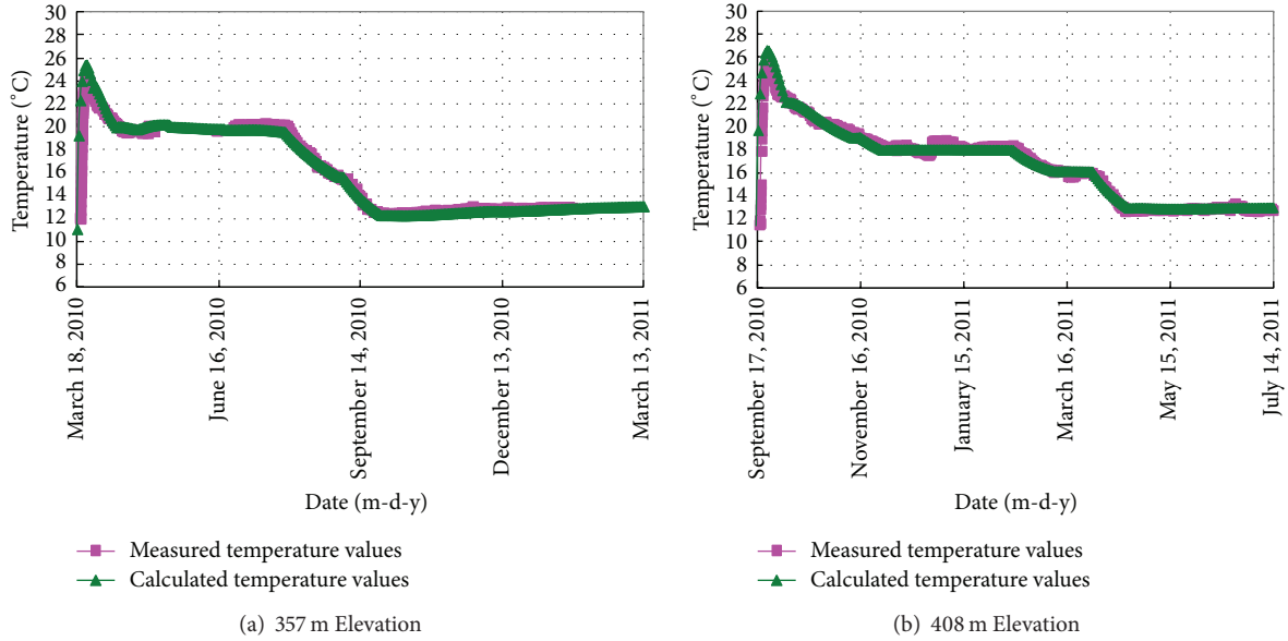
FIGURE 5: Comparisons between computational temperatures and measured ones.
