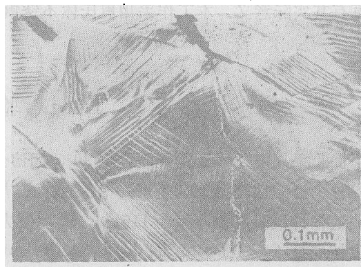
图 2 裂纹在过载塑性区内的扩展 Fig. 2 Propagation of a crack in overload plastic zone
